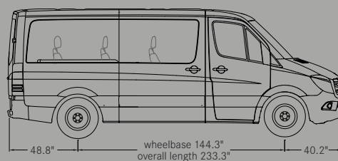
144" WHEELBASE
