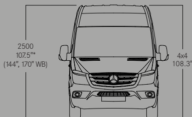
HIGH ROOF
